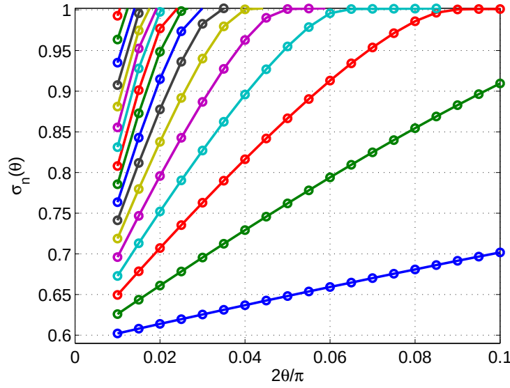
Figure 2: \sigma_n(\theta; 100, 100, 50) for n = 1, \dots, 17 (ordinates) versus \vartheta = 2\theta/\pi (abscissa). Sampling: \vartheta = k/200 , 2 \leq k \leq 20 .
