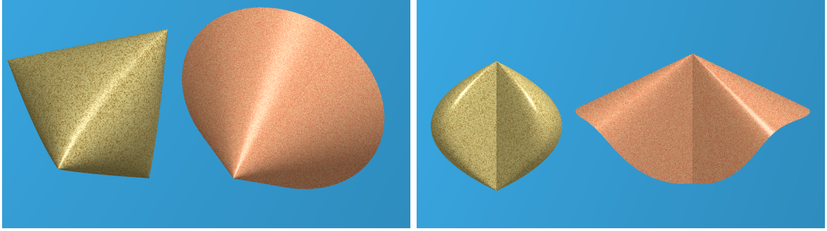
(A) The Cayley tetrahedron
