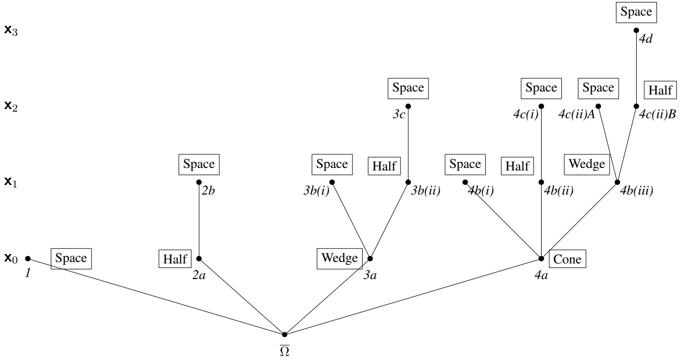
FIGURE 3.3. The tree of singular chains with numbering according to Description 3.32 (Half is for half-space)
