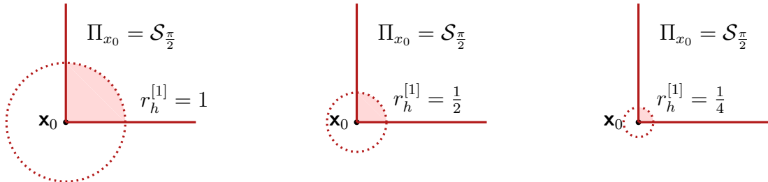
FIGURE 9.2. Support of sitting quasi-modes
