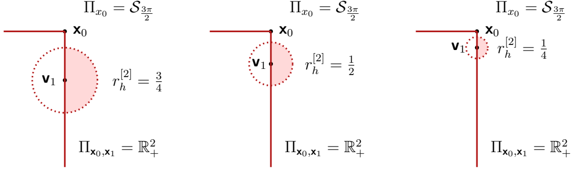
FIGURE 9.3. Sliding quasi-modes
