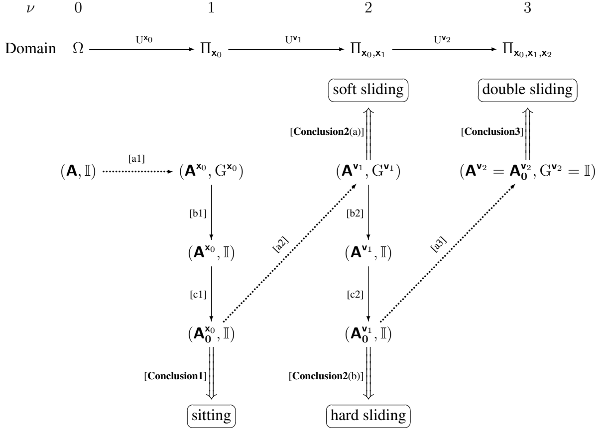
FIGURE 9.1. Construction of quasimodes
