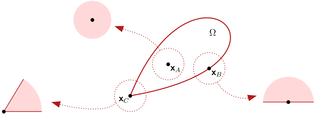
FIGURE 3.1. Tangent sectors for a curvilinear polygonal domain
