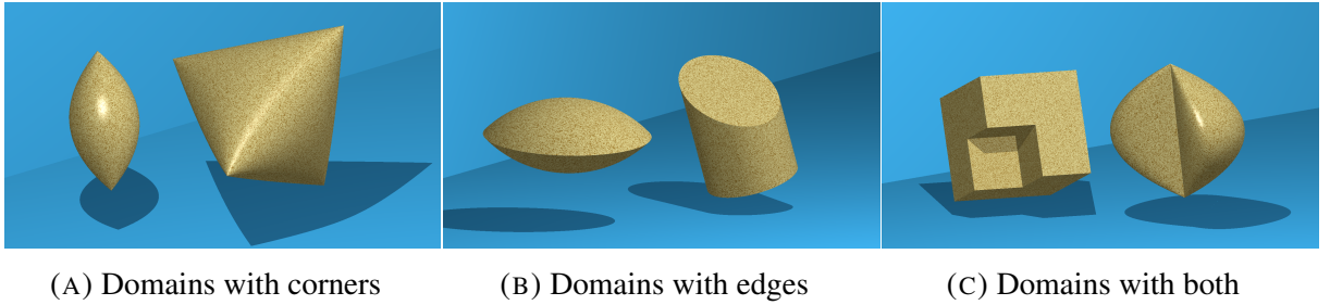
FIGURE 1.1. Examples of 3D corner domains (Figures drawn by M. Costabel with POV-ray)
