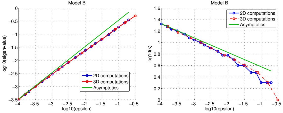
FIGURE 8. Model B: First eigenvalue \tilde{\lambda}_1^\varepsilon and associated azimuthal frequency k(\varepsilon) .
