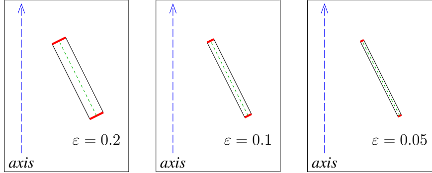
FIGURE 7. Model B: Meridian domains for several values of \varepsilon .
