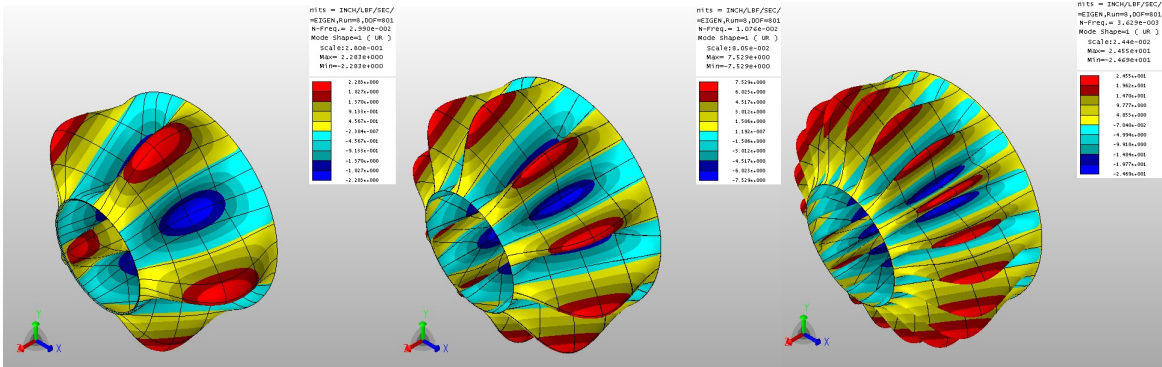
FIGURE 9. Model B: First eigenmode (radial component) for \varepsilon = 10^{-2}, 10^{-3}, 10^{-4} .
