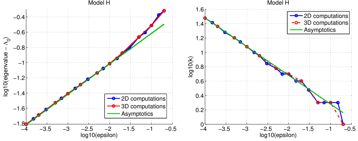
FIGURE 13. Model H: Difference \tilde{\lambda}_1^\varepsilon - \Lambda_0 and associated azimuthal frequency k(\varepsilon) .
