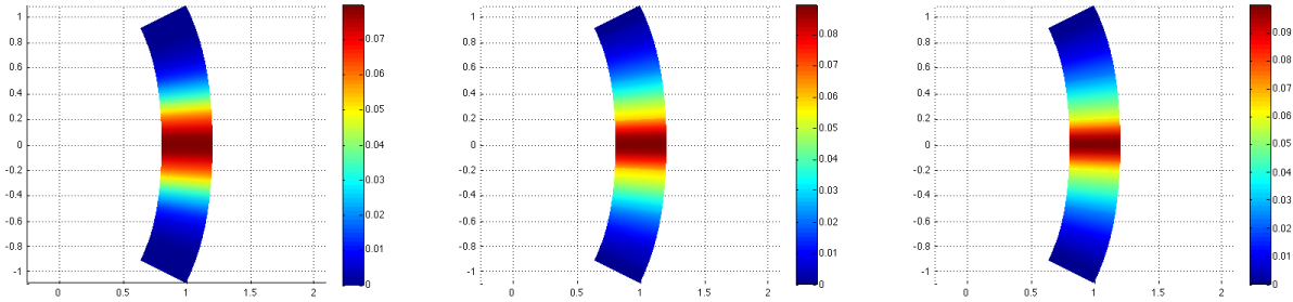
FIGURE 15. Model H: 2D first eigenmode (radial component) for \varepsilon = 10^{-3} and k = 12 , \varepsilon = 3 \cdot 10^{-4} and k = 19 , \varepsilon = 10^{-4} and k = 30 . Represented on \omega^{0.2} .
