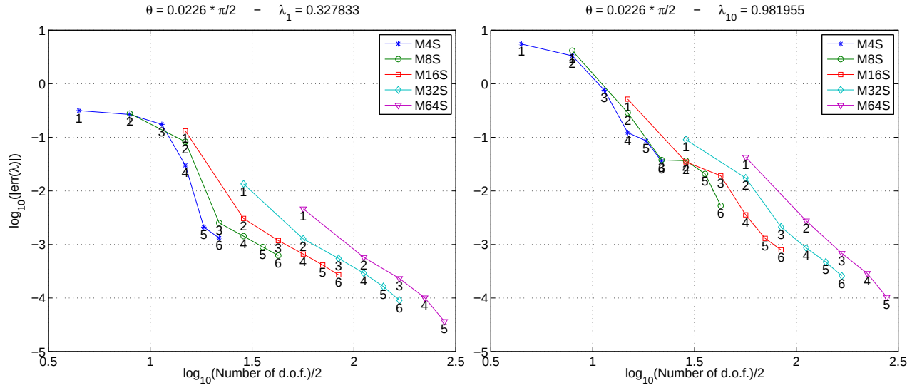
FIGURE 23. Convergence towards \lambda_1 \simeq 0.32783 and \lambda_{10} \simeq 0.98195 .
